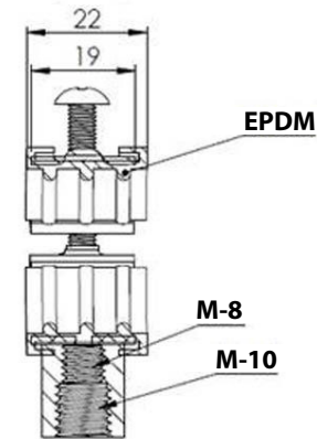
SECTION L-L
